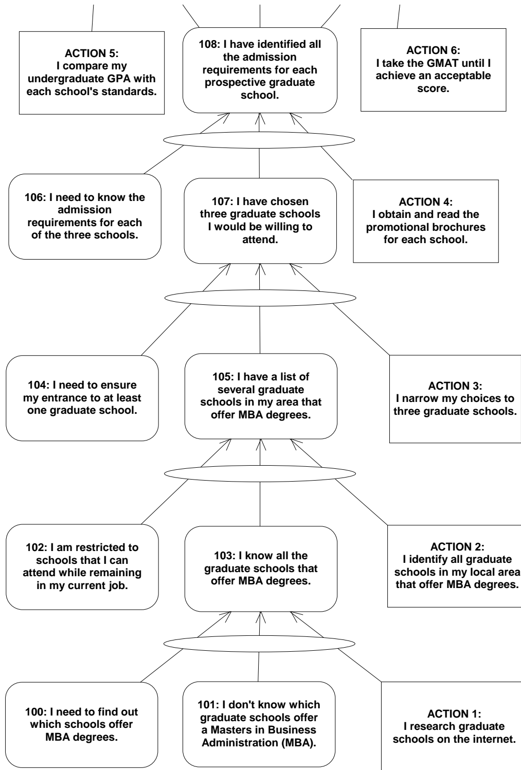
Figure 10.9.1 Completing the transition tree: Step 4.
